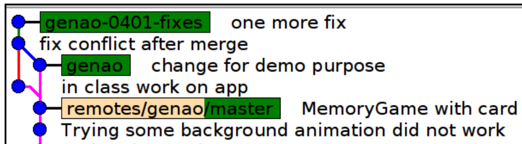
Figure 1: Branch and merge example
